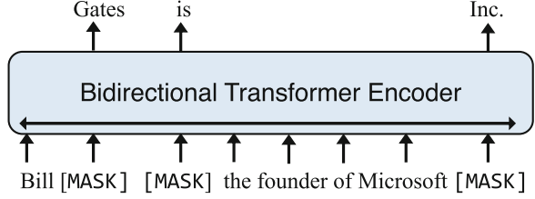
Fig. 5.4 The masked language model objective
