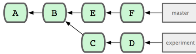
Figure 6.1: Example history for range selection.
