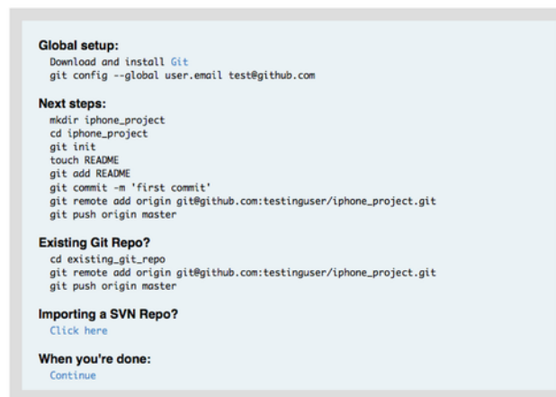
Figure 4.7: Instructions for a new repository.
