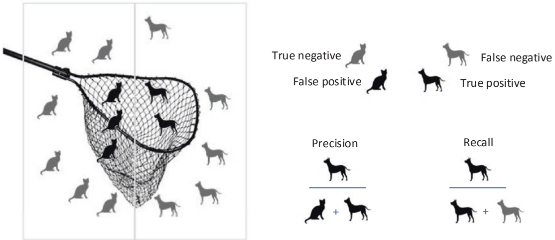
Figure 4-2. Precision and recall for a dog catcher
