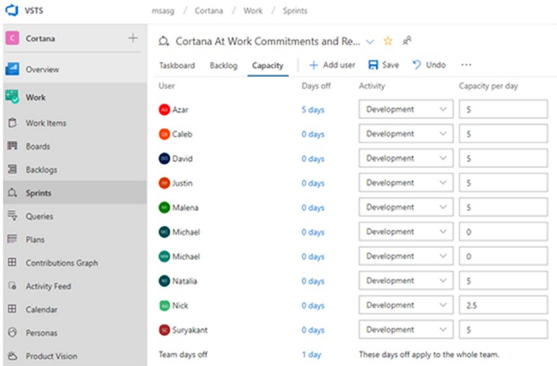
Figure 4-12. Azure DevOps Capacity tab
